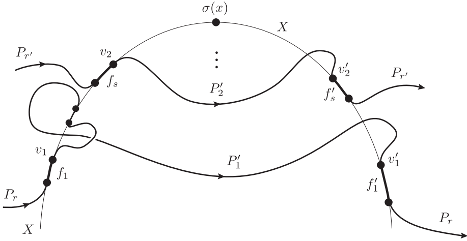
Figure 3. Constructing the paths P'_i
